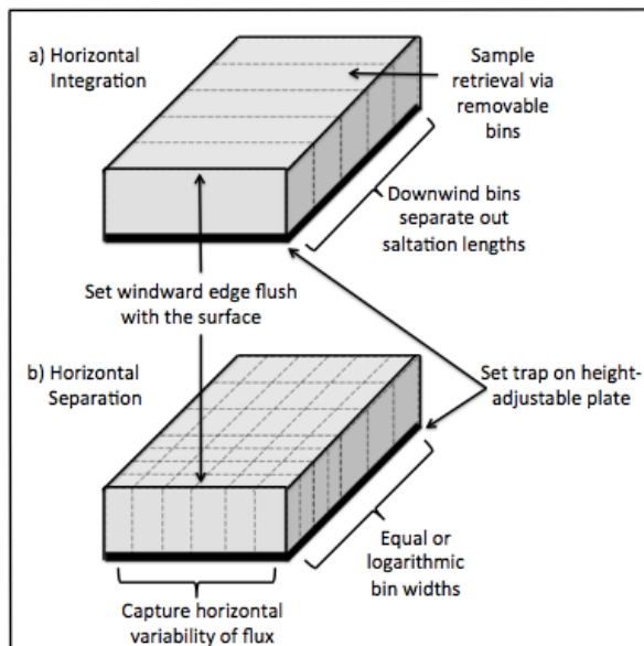
Figure 4: This figure illustrates the design and suggested deployment strategies for horizontal saltation traps. These traps should be buried in, and set flush with, the surface. a) Shows a horizontally integrating saltation trap 2m long and 0.20m wide (dimensions based on Namikas, 2003), and b) shows a horizontal- and streamwise-separated saltation trap.
