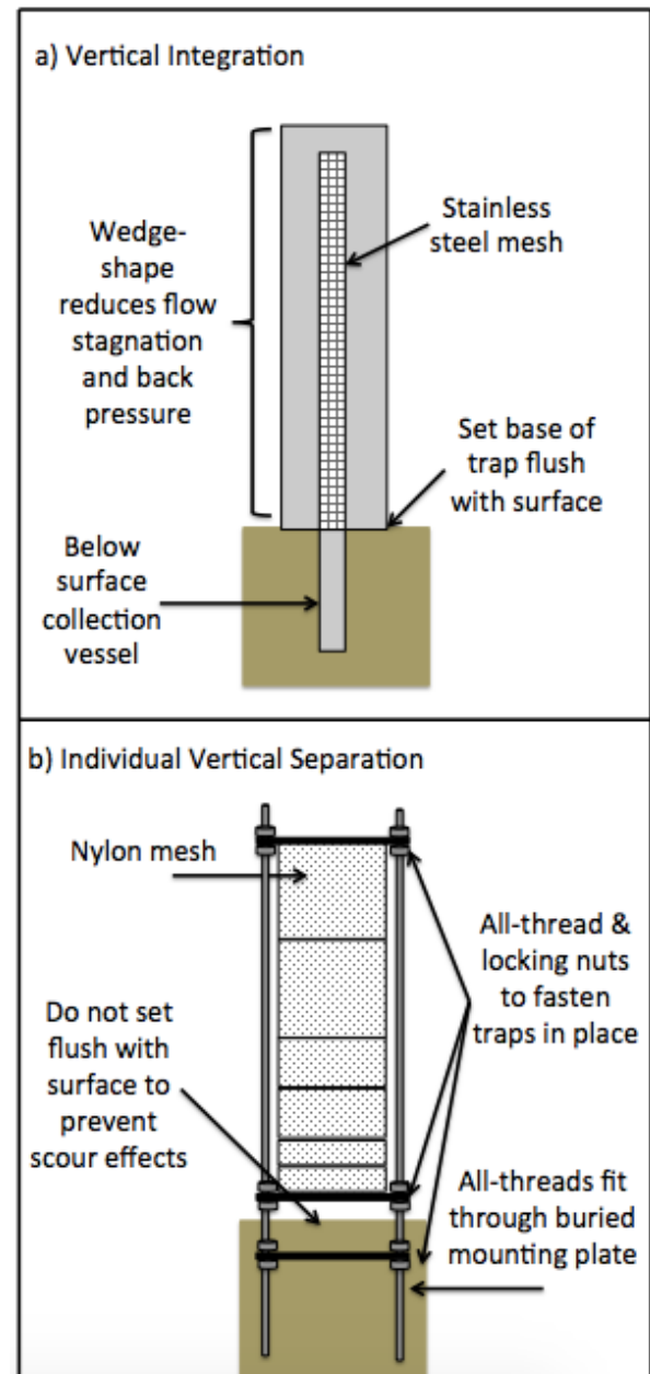
Figure 3: This figure illustrates the design and suggested deployment strategies for vertical saltation traps. In this figure the windward profile of the traps are drawn. a) Shows a vertically integrating saltation trap, and b) shows a height-separated vertical saltation trap.
